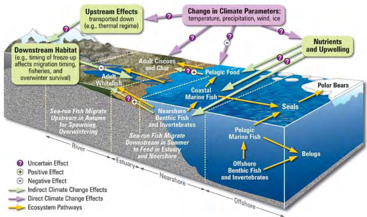
Figure 15. A stylized portrayal of some potential direct effects of climate parameters on arctic aquatic environments and some potential indirect effects on aquatic organisms (such as anadromous fish). The complexity of interactive effects raises great difficulties in projecting climate change effects on these fishes. Source: Reist et al.2006. [32]
