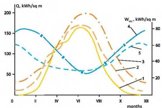
Pic. 3.4 An annual cycle of mean monthly global solar radiation (Q, in kilowatt-hours per square meter) in the polar (1), middle (2) and southern (3) latitude; an annual cycle of potential energy production at a wind energy converter (W wec , in kilowatt-hours per square meter) on the northern (4) and southern (5) coasts of Kola Peninsula 1-Khibiny station; 2 – Minsk; 3 – Sochi; 4 – Dalniye Zelentsy; 5 – Chavanga.
