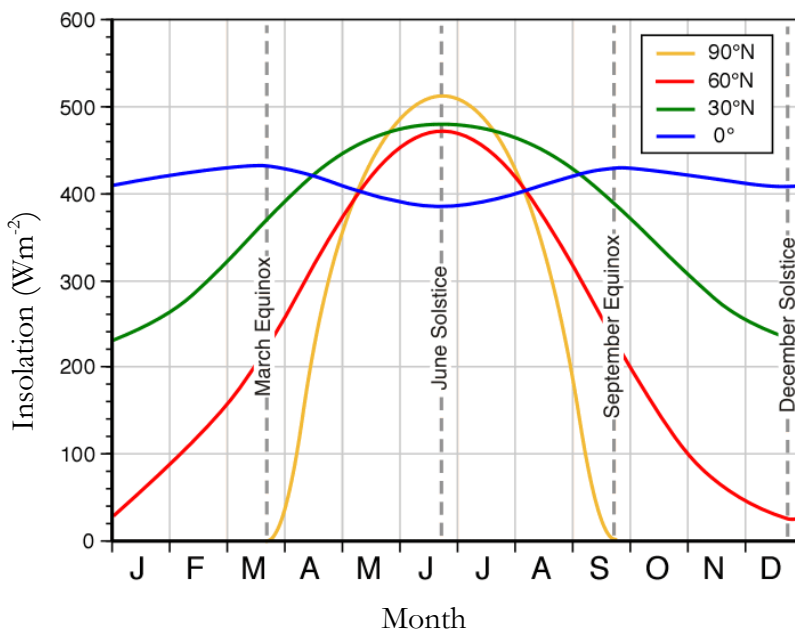
Figure 12. Monthly values of available insolation in \text{Wm}^{-2} for the equator, 30^{\circ} , 60^{\circ} , and 90^{\circ} North over a one-year period.
