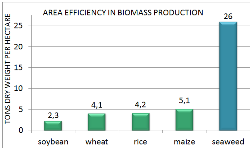
Figure 7: Area efficiency of marine and land plants measured in dry weight per hectare.
